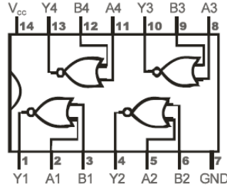
7402 Quad 2-Input NOR Gate
