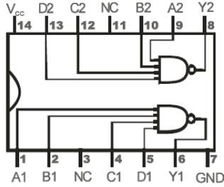
7420 Dual 4-Input NAND Gate
