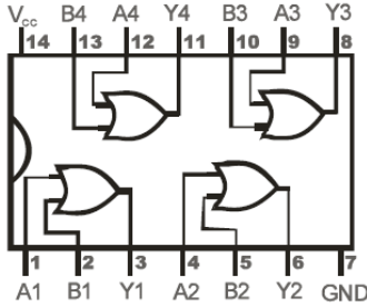
7432 Quad 2-Input OR Gate
