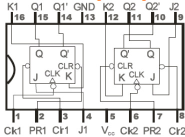
7476 Dual J-K Flip-Flop
