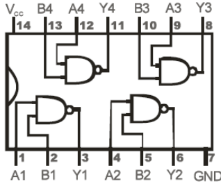
7400 Quad 2-Input NAND Gate
