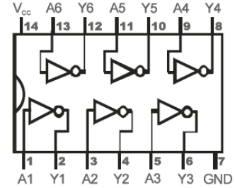
7404 Hex Inverter
