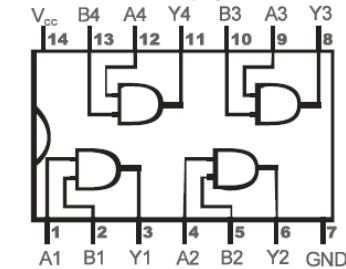
7409 Quad 2-Input AND Gate (Open Collector)
