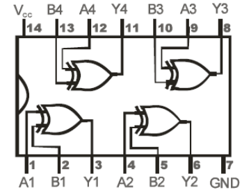
7486 Quad 2-Input XOR Gate
