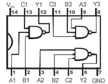
7410 Triple 3-Input NAND Gate
