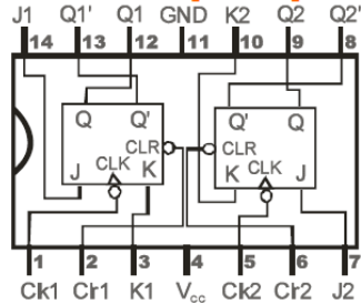
7473 Dual J-K Flip-Flop
