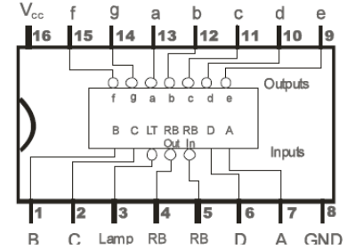
7447 Binary-to-BCD Converter
