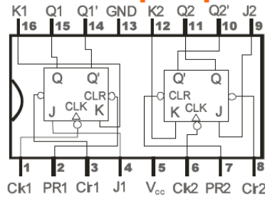
7476 Dual J-K Flip-Flop
